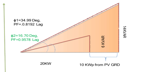
Fig-3 Vector diagram for P.F Improvement
