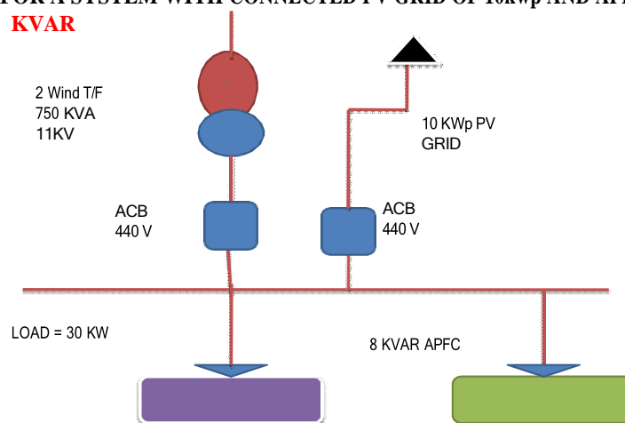
Fig.1 Block diagram for proposed system
