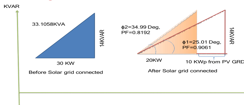
Fig-2 Vector diagram PF Reduction
