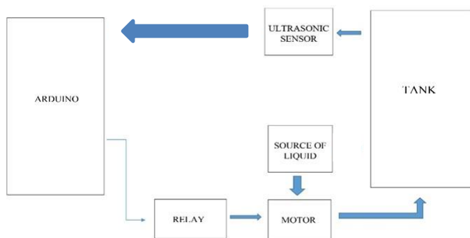
Fig 12: Block Diagram of Water Pumping System
