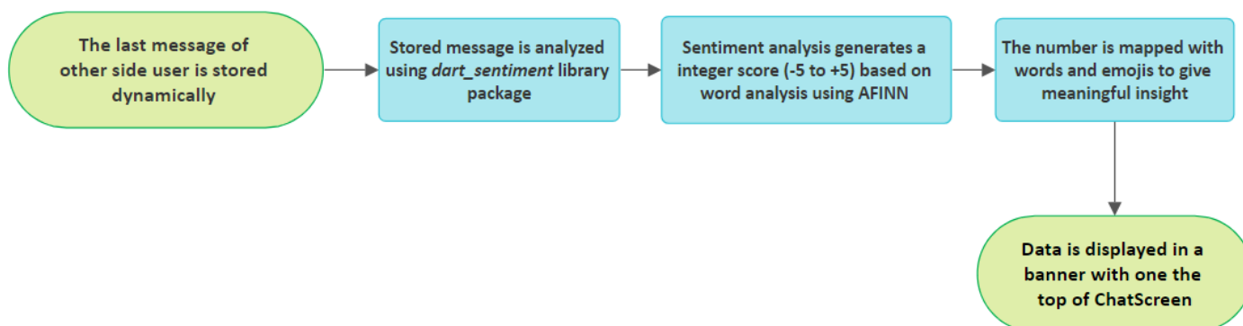
Figure 5: Working process of dart_sentiment
