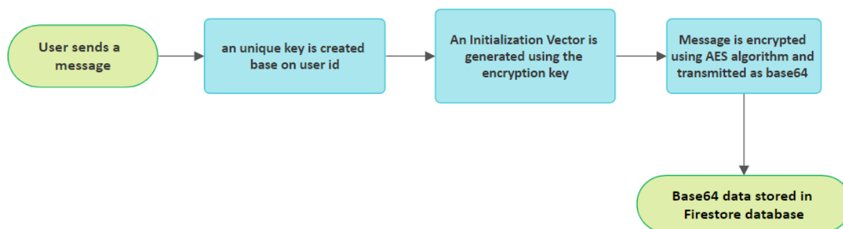
Figure 3: Encryption process
