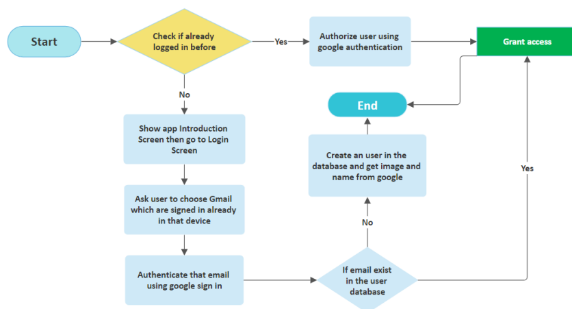
Figure 1: Flowchart of login process
